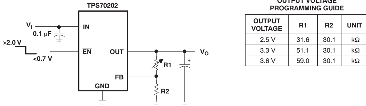
Figure 40. TPS70202 Adjustable LDO Regulator Programming
